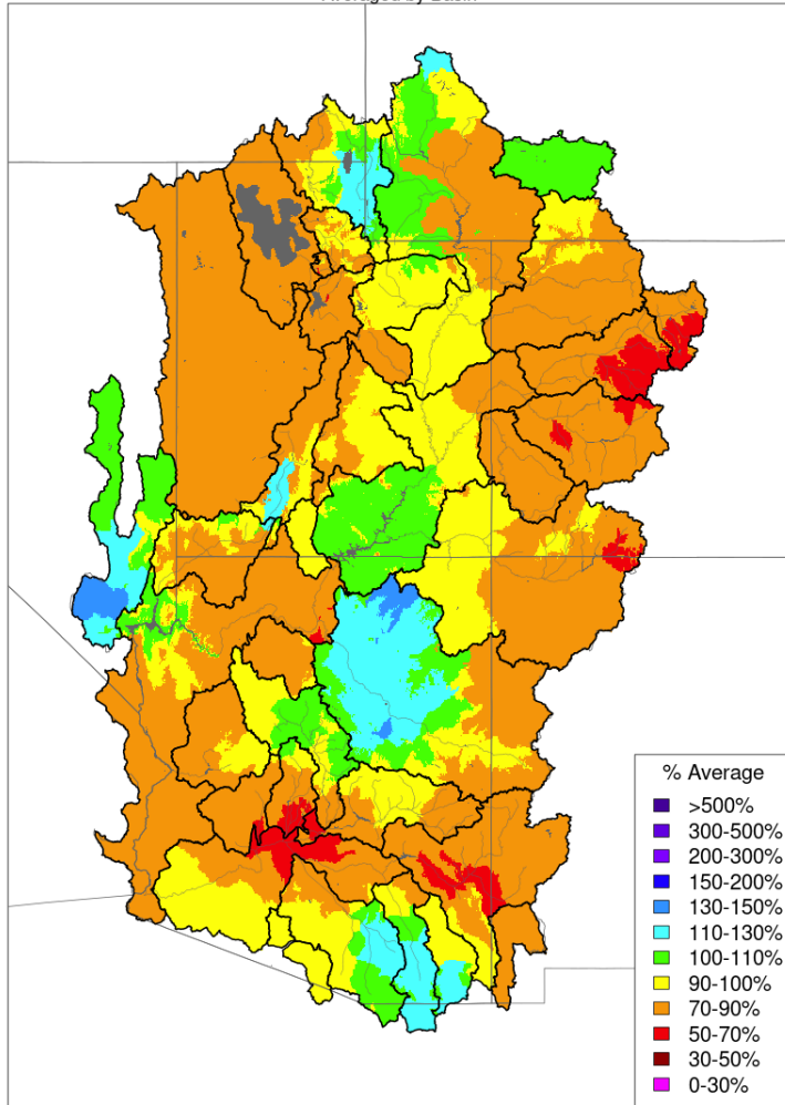
Water Year Precipitation, October 2025 - August 2026
