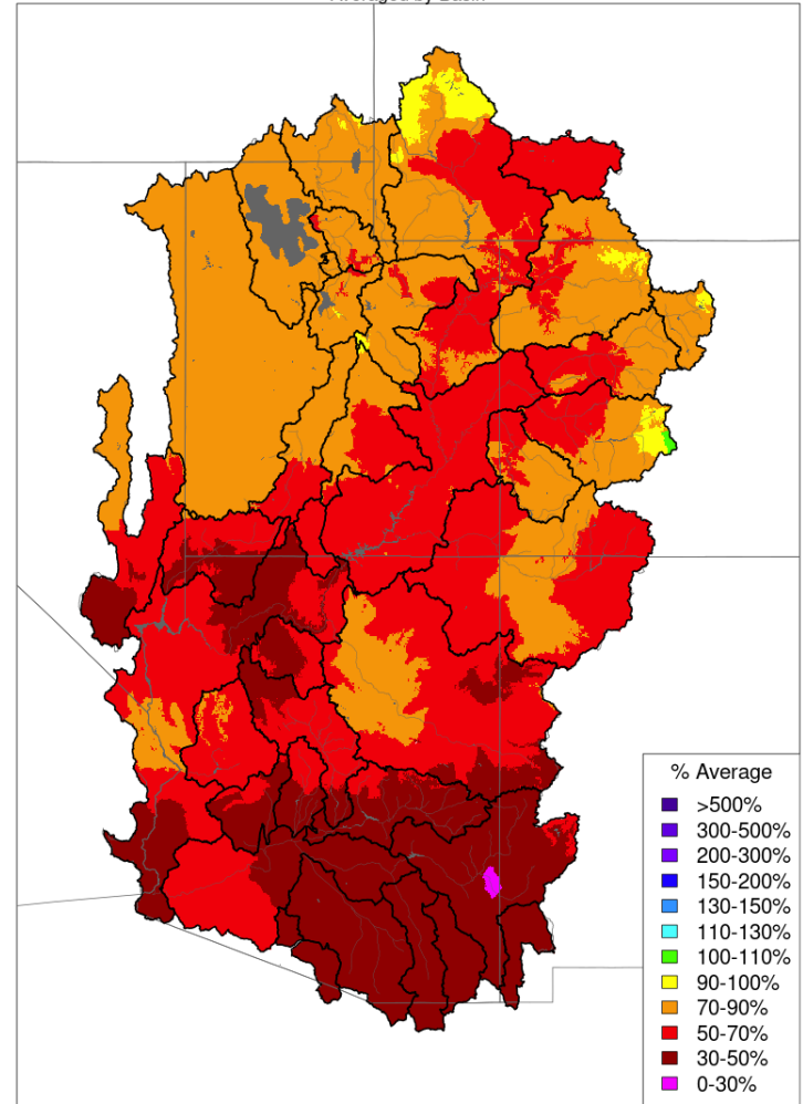
Water Year Precipitation, October 2024 - August 2025
