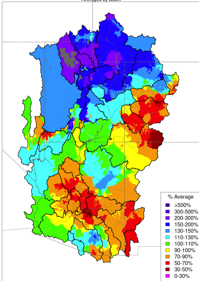
Monthly Precipitation - August 2026
