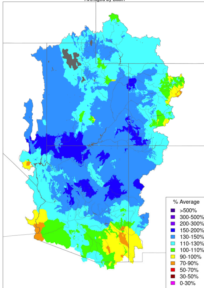
Water Year Precipitation, October 2022 - June 2023
