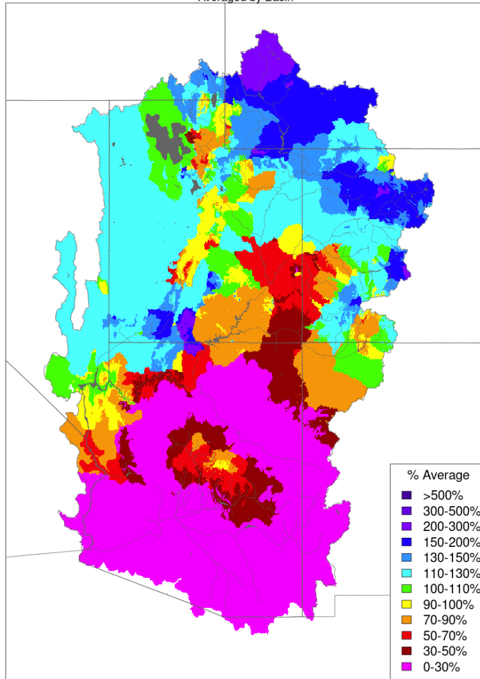
Monthly Precipitation - June 2023 Averaged by Basin
