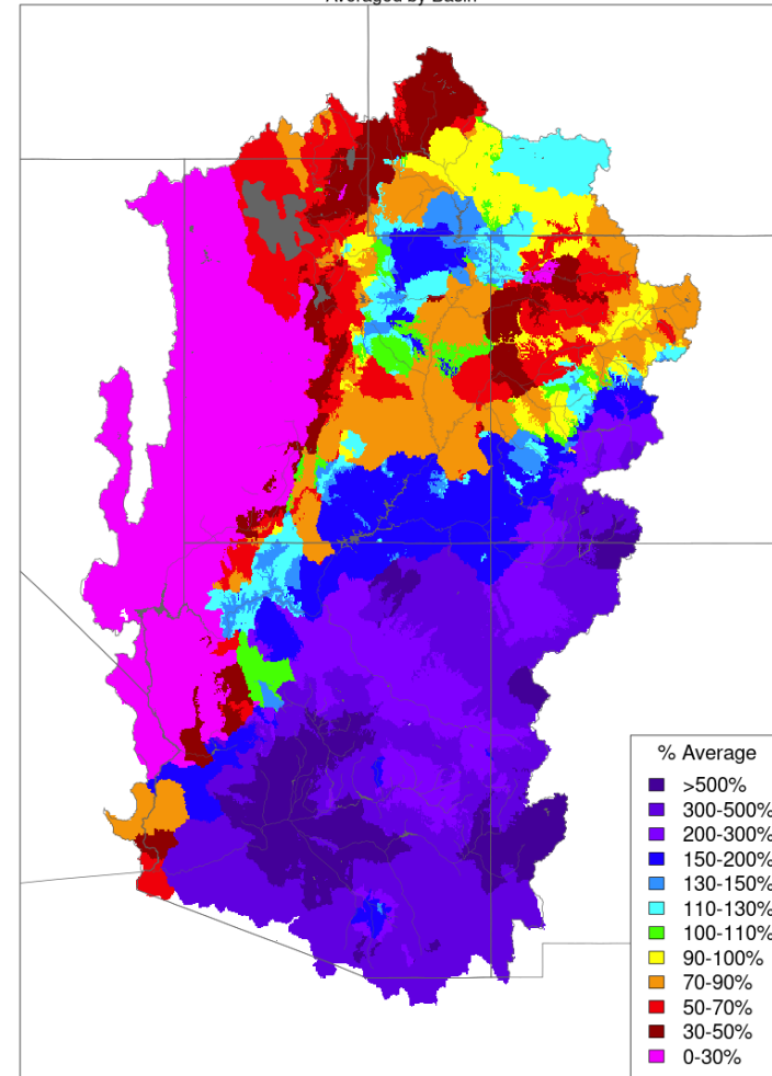
Monthly Precipitation - June 2022 Averaged by Basin
