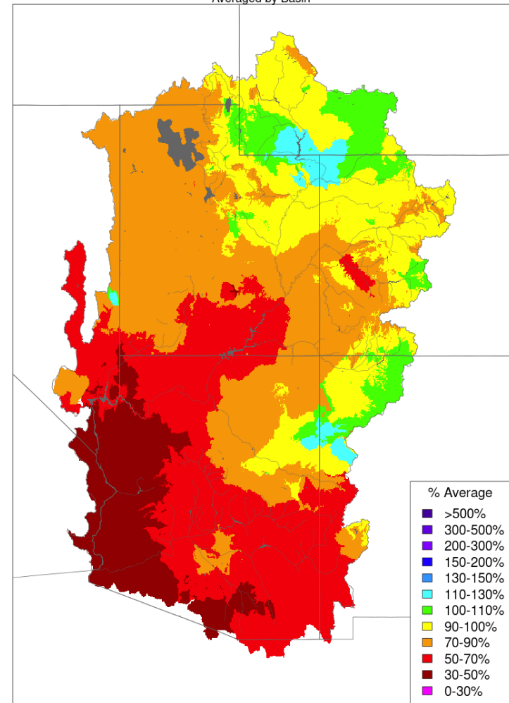
Water Year Precipitation, October 2021 - June 2022
